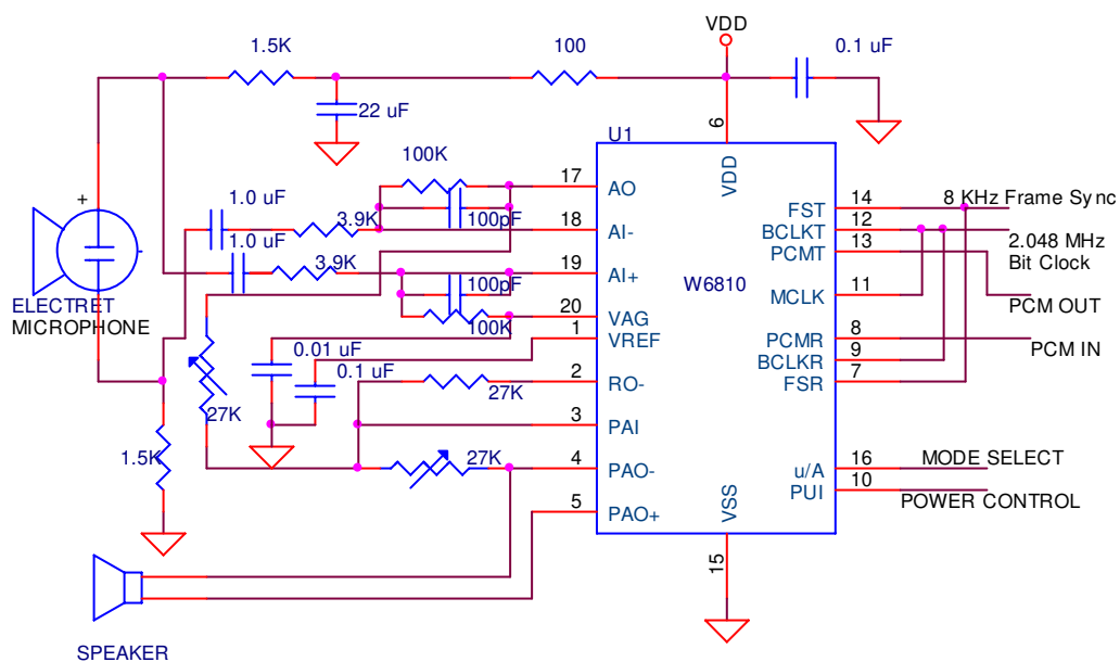
Figure 11.3 Handset Interface
